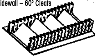
2 Sidewall - 60° Cleats
