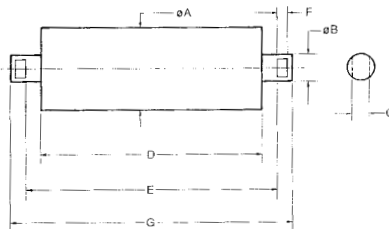
ROLLER DIMENSIONS FOR ORDERING
