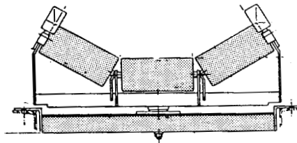
TRAINING TROUGH SET
